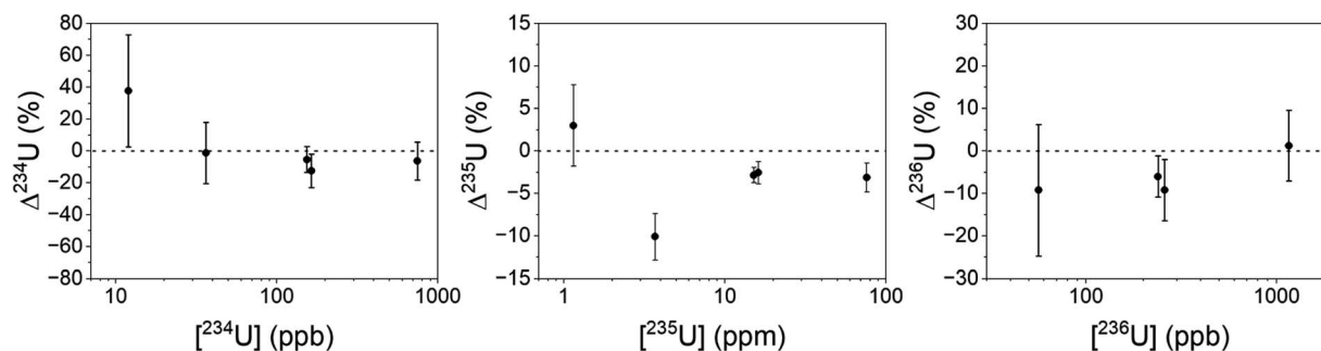
Fig. 5 Uranium isotope ratios ( ^x\text{U}/^{238}\text{U} ) as a function of the amount of the minor isotopes of U in the samples. Repeated measurements are slightly offset from one another in concentration for clarity. Uncertainties are 1\sigma .
