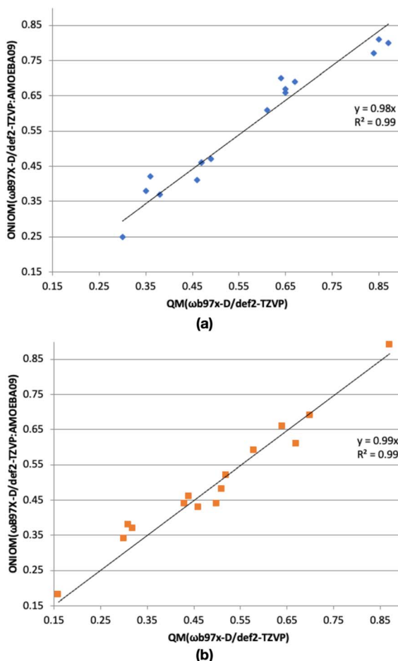
Fig. 4 ONIOM( \omega\text{B97X-D/def2-TZVP:AMOEB}09 ) binding energy (without ZPE) vs. \omega\text{B97X-D/def2-TZVP} binding energy (without ZPE) of (a) \text{CH}_2\text{OH} radical, and (b) \text{CH}_3\text{OH} . Intercept of the linear trendlines were set to 0.0.
