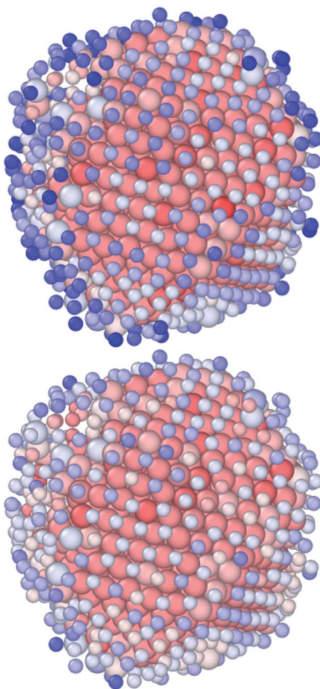
Fig. 4 Au 283 Pt 1132 NAs where atoms are coloured based on their nominal CN (top, with a cutoff of 3.55 Å) and the VMCN (bottom). Atoms are coloured with respect to their CN (or VMCN), ranging from 16 (full red) to 3 (dark blue). Au atoms are represented as smaller than Pt, to improve visualization. Minor discrepancies between the two algorithms occur. Using the solid angle condition, we count 561 atoms with a CN less than 10, 170 with CN = 11, and 684 with a CN above or equal to 12; using van Meel's algorithm, their occurrence is 477, 216, and 722, respectively.
