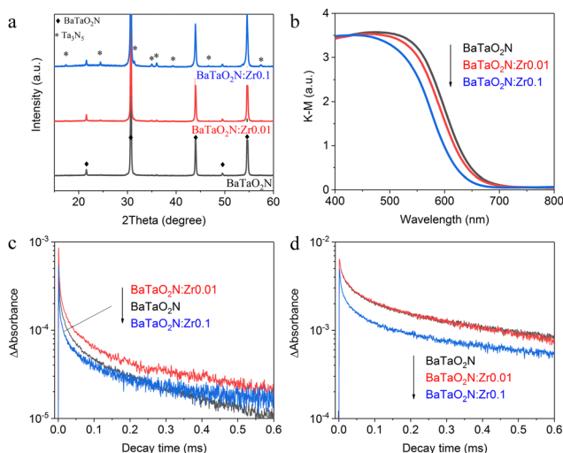
Fig. 2 (a) XRD patterns, (b) DRS spectra, and TAS decays probed at (c) 5000 \text{ cm}^{-1} (2000 nm; corresponding to electron dynamics) and (d) 15400 \text{ cm}^{-1} (649 nm; corresponding to hole dynamics) with excitation at 470 nm for BaTaO 2 N, BaTaO 2 N:Zr0.01 and BaTaO 2 N:Zr0.1.
