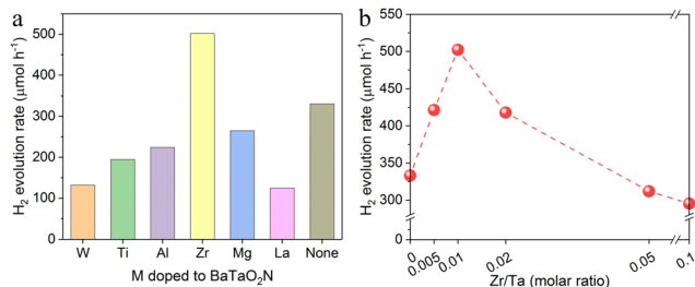
Fig. 1 Photocatalytic \text{H}_2 evolution rates obtained for (a) Na–Pt/BaTaO 2 N doped with various cations (M) with a M/Ta ratio of 0.01 and (b) Na–Pt/BaTaO 2 N:Zr with different Zr/Ta molar ratios in an aqueous solution containing methanol (15 vol%). Reaction conditions: 0.23 wt% Na 0.3 wt% Pt/BaTaO 2 N photocatalyst, 100 mg; 15 vol% aqueous methanol solution, 150 mL; light source, 300 W Xenon lamp equipped with a cut-off filter ( 420 \text{ nm} < \lambda < 800 \text{ nm} ). Reaction system, Pyrex top-illuminated vessel connected to a closed gas-circulation system with a 10 kPa Ar background pressure.
