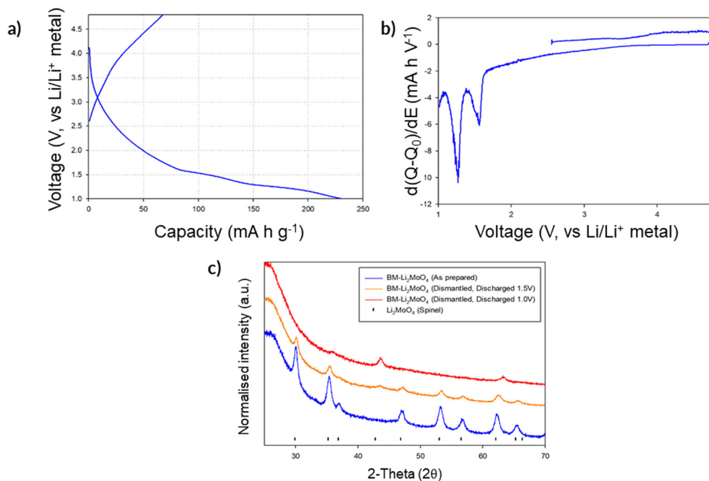
Fig. 7 (a) First cycle voltage profile for \text{BM-Li}_2\text{MoO}_4 cycled in the region of 4.8–1.0 V at 10 \text{mA g}^{-1} ; (b) associated dQ/dV plot of the first charge/discharge cycle; (c) PXRD of dismantled swagelok cells showing phases formed once discharged down to 1.5 and 1.0 V (Cu K \alpha ).
