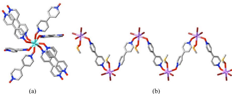
Fig. 10 Differing stoichiometry in complexes of 4,4'-bpdo: (a) the eight-coordinate \text{La}(\text{III}) centre in the diperiodic polymer [\text{La}(\text{L20})_4](\text{ClO}_4)_3 (CCDC 239608 85 ) where all ligands bridge in a bis( \kappa^1\text{O} ) manner to other \text{La}(\text{III}) ions (not shown). (La = sky blue); (b) similar bridging of \text{Bi}(\text{III}) centres in the monoperic polymer [\text{BiBr}_3(\text{dmsO})(\text{L20})] (CCDC 2008674 73 ). (Bi = violet, Br = brown, S = orange; partial disorder of the dmsO ligands not shown.)
