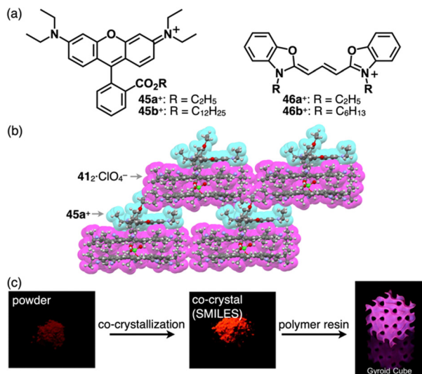
Fig. 31 (a) Rhodamines 45a + , 45b + and cyanines 46a + , 46b + , (b) single-crystal X-ray structure of 45a + · 41 2 ·ClO 4 - (redrawn from a cif file: 1895155) and (c) photographs of 45a + (left), 45a + · 41 2 ·ClO 4 - (centre) and 45a + · 41 2 ·ClO 4 - contained in polymer resin (right) (redrawn from ref. 76c. Copyright 2020 Elsevier).
