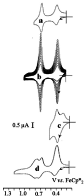
Fig. 17 Selective roles of the inner and outer ferrocenyl redox centers of the 81-biferoceyl dendrimer in the redox recognition of \text{ATP}^{2-} and \text{Pd}^{2+} . Cyclic voltammograms of the G2-81-biferoceyl click dendrimer, (a) in \text{CH}_2\text{Cl}_2 , [\text{n-Bu}_4\text{N}][\text{PF}_6] 0.1M; (b) progressive adsorption upon scanning around the potential of the biFc area; (c) splitting of the outer-Fc CV wave at 0.4V upon addition of [\text{ATP}][\text{n-Bu}_4\text{N}]_2 ; (d) addition of \text{Pd}(\text{OAc})_2 provoking the splitting of the inner-Fc wave at 0.7 V. Reproduced with permission from ref. 117. Copyright 2010 Wiley-VCH.
