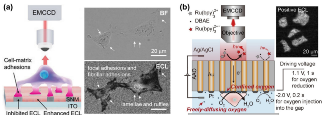
Fig. 2 (a) Schematic illustration of imaging cell–matrix adhesions by ECLM in the negative mode (left). The bright field (BF) and corresponding ECL image of cells (right). Reproduced from ref. 42 with permission from Wiley-VCH. (b) Scheme of ECL imaging of cell–matrix adhesions in the positive mode by using a closed bipolar nano-electrode array. Reprinted from ref. 45 with permission from Wiley-VCH.
