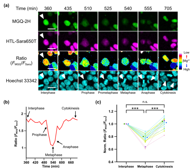
Fig. 3 (a) Confocal fluorescence imaging of intranuclear Mg^{2+} dynamics in HEK293T cells during mitosis. Scale bar: 20 \mu m. (b) Time course of fluorescence ratio ( F_{MGQ}/F_{Sara} ) of a mitotic cell indicated by an arrowhead in (a). (c) Quantitative analysis of the ratio during each stage of mitosis. A circular dot indicates each data point, and a rectangle dot indicates the median of each experiment ( n = 19 cells, 3 experiments). *** p < 0.001 . n.s.: not significant ( p = 0.61 ).
