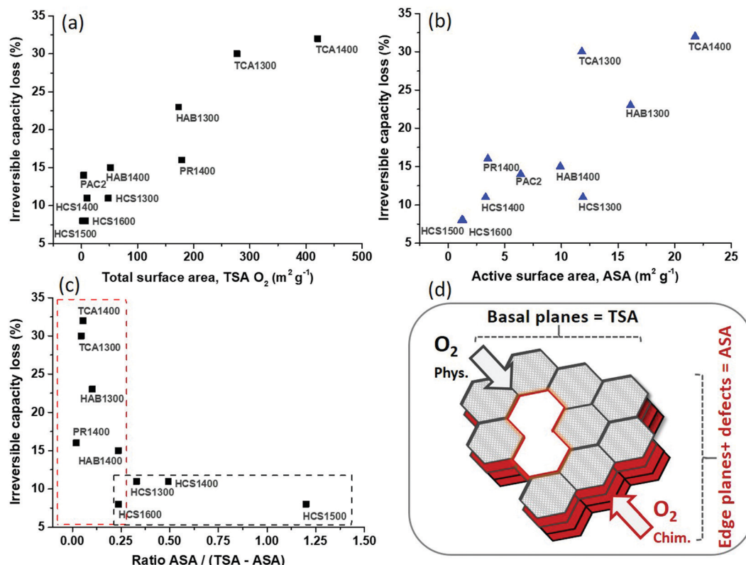
Fig. 3 Relationship between the 1st irreversible capacity loss and (a) total surface area (TSA O 2 ), (b) active surface area (ASA), (c) ratio ASA/(TSA - ASA). (d) Representation of hard carbon structure containing the active surface (edge planes and defects) and the basal planes surface (TSA-ASA).
