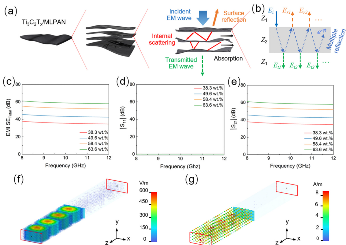
Fig. 5 Principle and electromagnetic simulations. (a) Schematic of the EMI shielding principle of the dual-scale multilayer Ti_3C_2T_x/MLPAN hybrid fabric. (b) Multiple reflections occurred inside monolayer Ti_3C_2T_x when the material thickness was lower than the corresponding skin depth, where \gamma is the propagation constant and t is the thickness of the material. Simulation results of (c) SE_{Total} , and the corresponding S -parameters include (d) |S_{11}| and (e) |S_{21}| . Field distribution simulation results for electromagnetic waves including the (f) electric field and (g) magnetic field.
