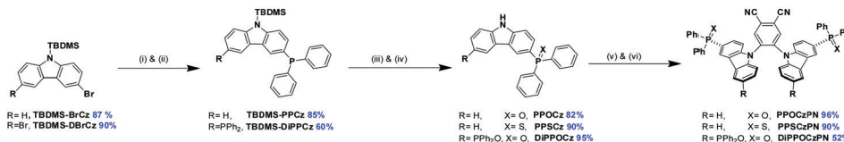
Scheme 2 Synthetic routes for the synthesis of PPOCzPN and DiPPOCzPN . Reaction conditions: (i) n -BuLi (1.6M), THF, -78 ^\circ\text{C} , 30 min, (ii) \text{PPh}_2\text{Cl} , -78 ^\circ\text{C} – rt, 30 min, (iii) \text{H}_2\text{O}_2 or \text{S}_8 , THF, rt, 18 h, (iv) TBAF (1.0 M), THF, rt, 1 h, (v) NaH, THF, 30 min, (vi) 4,5-difluorophthalonitrile, rt, 6 h.
