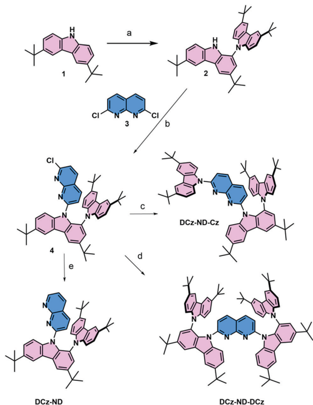
Scheme 1 Reagents and conditions: (a) [\text{Ru}(p\text{-cymene})\text{Cl}_2]_2 , dppe, \text{Cu}(\text{OAc})_2 , \text{PhCl} , 1,1,2,2-tetrachloroethylene, \text{AcOH} , \text{O}_2 , 150 °C, 82%; (b) 2 , 3 , n\text{-BuLi} , THF, 80 °C, 86%; (c) 3,5-di- tert -butylcarbazole, \text{NaH} , THF, 80 °C, 88%; (d) \text{NaH} , THF, 40%; and (e) \text{Pd}(\text{OAc})_2 , \text{Bu}_4\text{NBr} , DMF, i\text{PrOH} , 115 °C, 36%.
