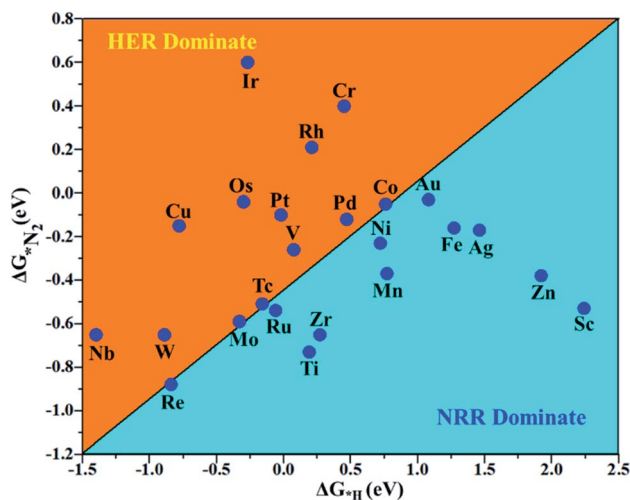
Fig. 4 Calculated Gibbs free energies of N_2 and H_2 adsorbed on the M_1/\text{PMA} cluster, which are divided into the eNRR region ( \Delta G_{H^*} > \Delta G_{N_2} ) and HER region ( \Delta G_{H^*} < \Delta G_{N_2} ).
