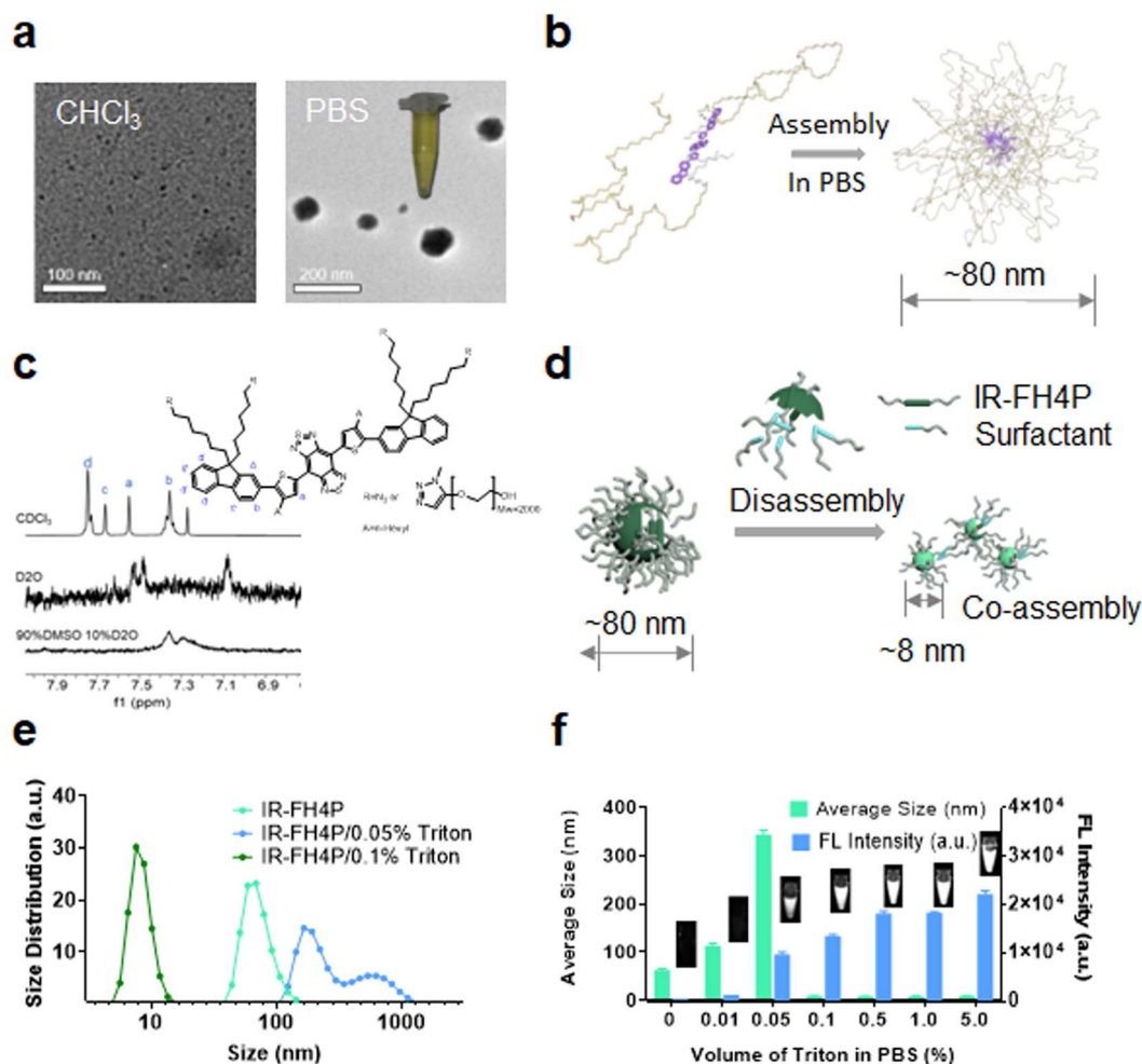
Fig. 2 Self-assembly of IR-FH4P in PBS and disassembly of surfactant-chaperoned dye system. (a) TEM image of IR-FH4P (10 \mu M) in \text{CHCl}_3 and PBS solution. (b) 3D model of IR-FH4P assembly in PBS. (c) ^1\text{H-NMR} spectra of IR-FH4P (1 mg) in \text{D}_2\text{O} , 90% DMSO-10% \text{D}_2\text{O} , and \text{CDCl}_3 , respectively. (d) 3D model of IR-FH4P disassembly and subsequently co-assembly with surfactant molecules. (e) DLS size distribution of IR-FH4P (10 \mu M) with modified Triton-X100 concentration. (f) Dynamic light scattering (DLS) analysis and NIR-II brightness of IR-FH4P (10 \mu M) with changing Triton-X100 concentration. All data are expressed as mean \pm SD.
