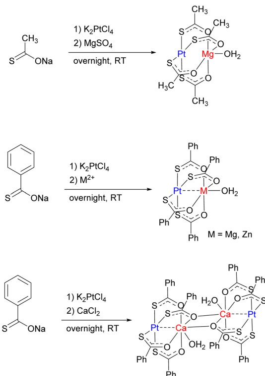
Scheme 20 Lantern Pt/M complexes with thiocarboxylate ligands.
