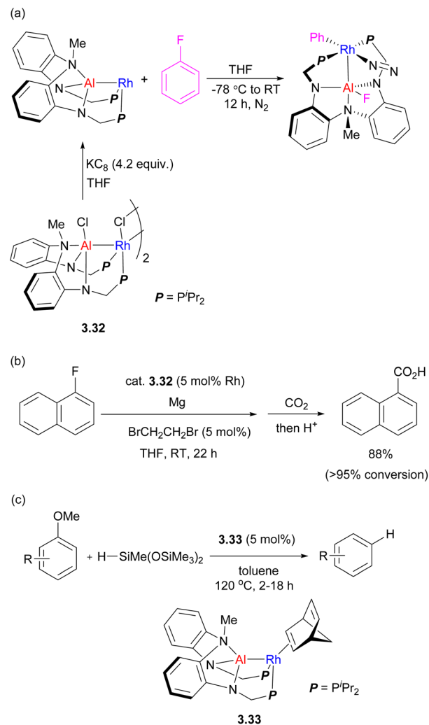
Scheme 27 (a) Fluorobenzene activation by an Al/Rh heterobimetallic complex. (b) Rh/Al catalyzed aryl fluoride magnesiation. (c) Catalytic C–O bond reduction catalyzed by Rh/Al complex.
