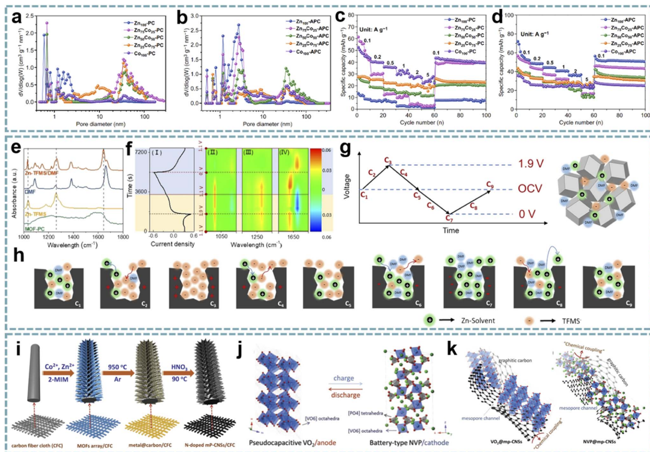
Fig. 7 MOF-derived porous carbons for MIHCs. Pore size distribution curves of (a) Zn_{100} -PCs and (b) Zn_xCo_{100-x} -APCs. Rate capabilities at different current densities of (c) Zn_xCo_{100-x} -PCs and (d) Zn_xCo_{100-x} -APCs. Reproduced with permission from ref. 160. Copyright 2020, Springer. (e) FT-IR spectra of neat DMF, Zn-TFMS, MOF-PC, and Zn-TFMS/DMF electrolytes. (f) CV curve (I) at 0.5\text{ mV s}^{-1} ; 2D color-filled contour plots (II, III, and IV) from the in situ ATR-FTIR test of the ZIHC. (g, h) The reaction process schematic diagram of the adsorption/desorption of ions in the MOF-PC electrode in a Zn-TFMS/DMF electrolyte. Reproduced with permission from ref. 161. Copyright 2021, Wiley-VCH. (i) Schematic diagram of the fabrication of N-doped mesoporous graphitic carbon nanosheet arrays. (j) Schematic illustration of the NIC device using flexible VO_2@mp\text{-CNSs/CFC} and NVP@mp\text{-CNSs/CFC} electrodes as the anode and cathode. (k) Schematic illustration of Na^+ storage of VO_2@mp\text{-CNSs/CFC} and NVP@mp\text{-CNSs/CFC} . Reproduced with permission from ref. 70. Copyright 2018, Wiley-VCH.
