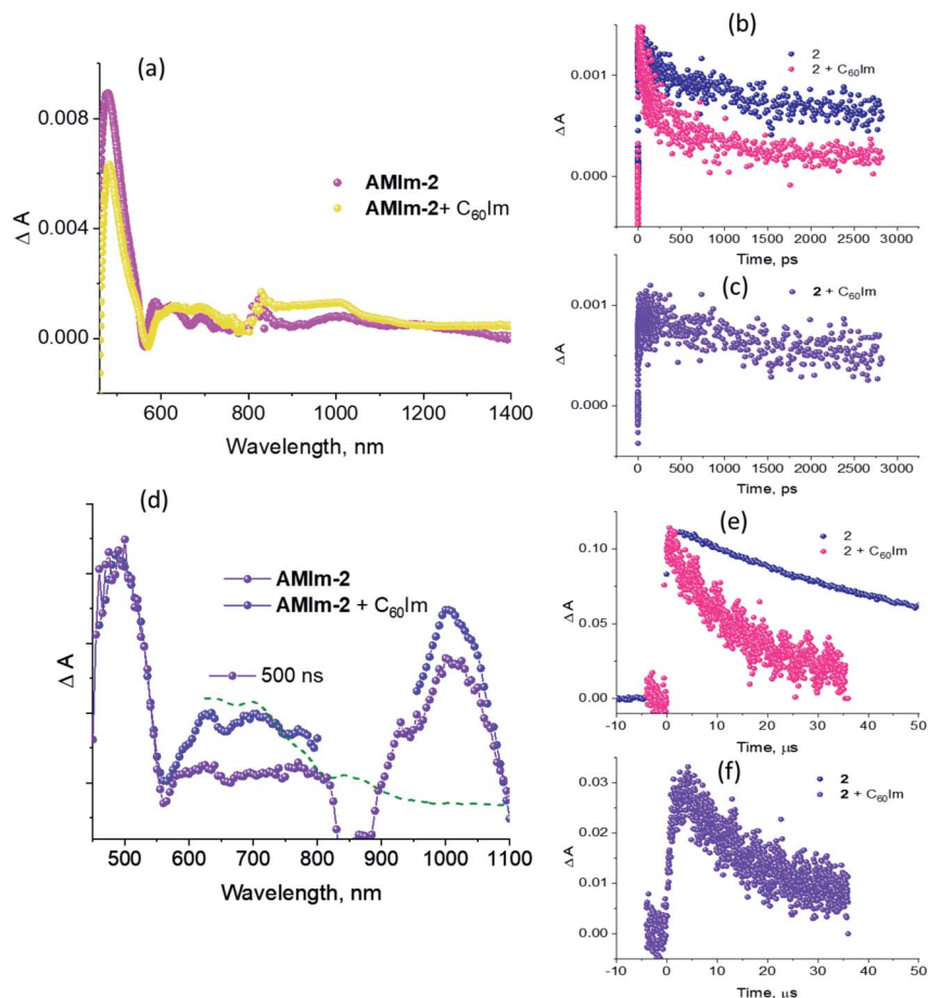
Fig. 9 (a) Fs-TA spectra of AMIm-2 and AMIm-2:ImC 60 complex in DCB at a delay time of 242 ps and an excitation wavelength of 420 nm. (b) Decay profile of the near-IR ESA peaks. (c) Decay profile of AMIm-2* + monitored at 695 nm for the dyad. (d) Nanosecond transient spectra, normalized to the 470 nm peak, of AMIm-2 and AMIm-2:ImC 60 complex in DCB at a delay time of 500 ns and an excitation wavelength of 420 nm. (e) Decay profile of the 470 nm peak corresponding to 3 AMIm-2*. (f) Decay profile of the AMIm-2* + monitored at 690 nm. The dashed line in (d) represents the spectrum of chemically oxidized AMIm-2 (NOBF 4 was used as an oxidizing agent).
