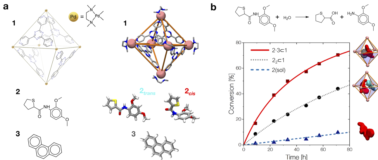
Fig. 1 The host–guest systems studied in this work. (a, top) The octahedral cage 1 used as a reference in this work is composed of four panel ligands (2,4,6-tris(4-pyridyl)-1,3,5-triazine) and six metal corners ( cis -endcapped Pd(II) complexes): chemical structure on the left and AA model on the right. (a, bottom) Chemical structure of amide guest 2 and of pirine co-guest 3 . AA models are reported on the right of each guest structure ( cis and trans isomers are shown for 2 ). (b, top) The hydrolysis reaction of the amide bond of 2 . (b, bottom) Experimentally observed percentage of hydrolyzed 2 over time. Conversion data are reported for the hydrolysis of 2 free in solution (in blue), in the case when two 2 guests are co-encapsulated in cage 1 (black), and for 2 co-encapsulated with co-guest 3 in cage 1 (in red: \sim 14\times hydrolysis acceleration compared to the blue curve). 10
