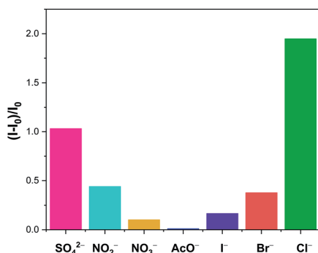
Fig. 10 Relative emission intensity increase of 10 \mu M tetraphenylthene AIE anion sensor 5.XB in the presence of 10 equiv. of various anions in THF. Reproduced from ref. 100 under the terms of the CC BY license.
