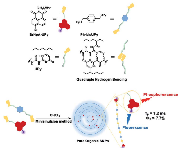
Fig. 19 Schematic illustration of the phosphorescence self-assembly of UPy-functionalized BrNpA-UPy.
