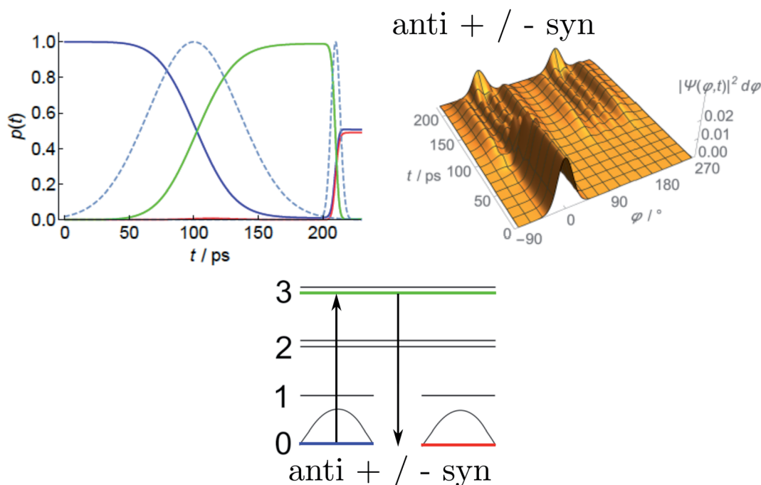
Fig. 30 Preparation of the exotic non-classical superpositions of the syn - and anti -isomer structures in m -o-phenol by a sequence of laser pulses. One starts in the localized ground state ( v_T = 0 ) of the more stable anti -isomer, which is excited by a first (long) laser pulse to the lower tunneling sublevel of the excited torsional state ( v_T = 3 ). This is a delocalized ‘tunneling switching’ state. A second, short laser prepares the superposition of syn - and anti -states in the v_T = 0 torsional level. The upper left shows the time dependent eigenstate populations (full lines) and laser pulses (dashed lines). The upper right part shows the wavepacket as probability |\Psi(\varphi, t)|^2 d\varphi as a function of the torsional angle. One recognizes the localized initial state, the delocalized intermediate state and the syn - and anti -superposition at the very end of the time range shown (after ref. 288).
