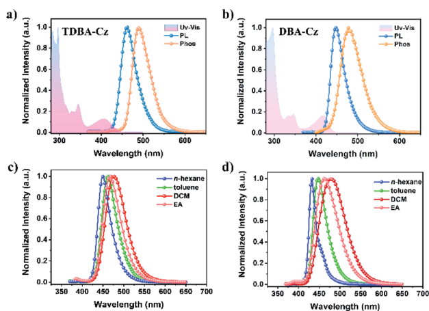
Fig. 2 Normalized UV-vis absorption, fluorescence (298 K) and phosphorescence (77 K) spectra of compounds (a) TDBA-Cz and (b) DBA-Cz in toluene solution ( 1 \times 10^{-5} M). PL spectra of neat films (c) TDBA-Cz and (d) DBA-Cz in different solvents.
