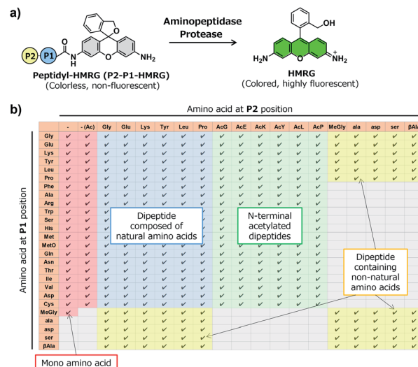
Fig. 1 Construction of a fluorescent probe library for aminopeptidases and proteases based on the HMRG scaffold. (a) Reaction scheme of peptidyl-HMRG with aminopeptidases or proteases. (b) List of the fluorescent probes in the library. Columns and rows represent amino acids at the P1 and P2 positions, respectively. Abbreviations: MeO; methionine sulfoxide.
