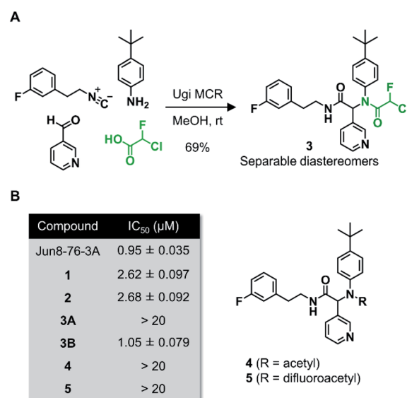
Fig. 2 (A) Preparation of the dipeptidic inhibitor 3 via Ugi multicomponent reaction (MCR). (B) Enzyme inhibitory activities of the dipeptidic inhibitors against SARS-CoV-2 M^{pro} . Compounds 3A and 3B are the less and more polar diastereomers, respectively. The reported IC_{50} values for Jun8-76-3A, 1 , and 2 are 0.31, 2.95, and 2.72 \mu M , respectively.
