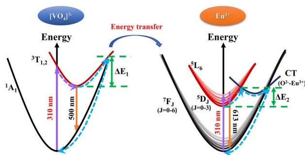
Fig. 9 Schematic configuration coordinate diagram for thermal-quenching of [\text{VO}_4]^{3-} groups and \text{Eu}^{3+} ions in LCZV host.
