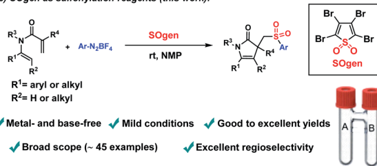
Fig. 1 Overview of tandem sulfonylative cyclization of 1,5-dienes: (a) sulfonyl chlorides as sulfonylation reagents; (b) sodium sulfonates as sulfonylation reagents; (c) SOgen as sulfonylation reagents (this work).
