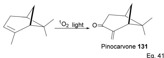
Scheme 35 Light-catalyzed oxygenation of pinene to pinocarvone.
