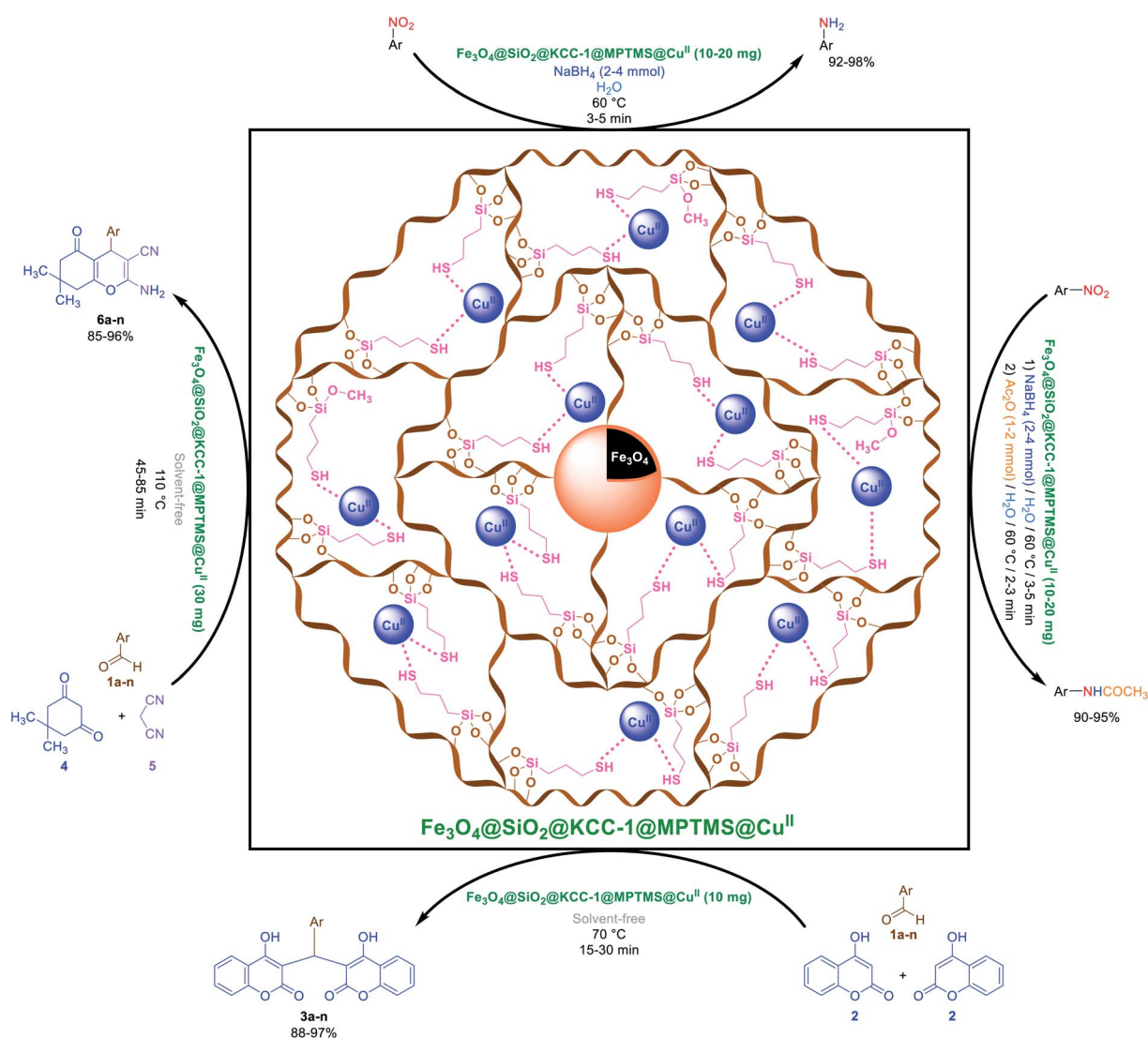
Fig. 1 Catalytic applications of the cockscomb flower-like Fe 3 O 4 @SiO 2 @KCC-1@MPTMS@Cu II mesoporous nanocomposite in the reduction and reductive acetylation of nitroarenes in water and solvent-free one-pot synthesis of some coumarin compounds.
