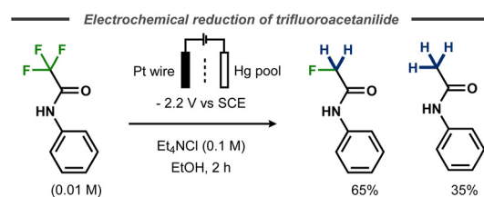
Fig. 20 Electrochemical defluorination of \alpha,\alpha,\alpha -trifluoroacetanilide. 72
