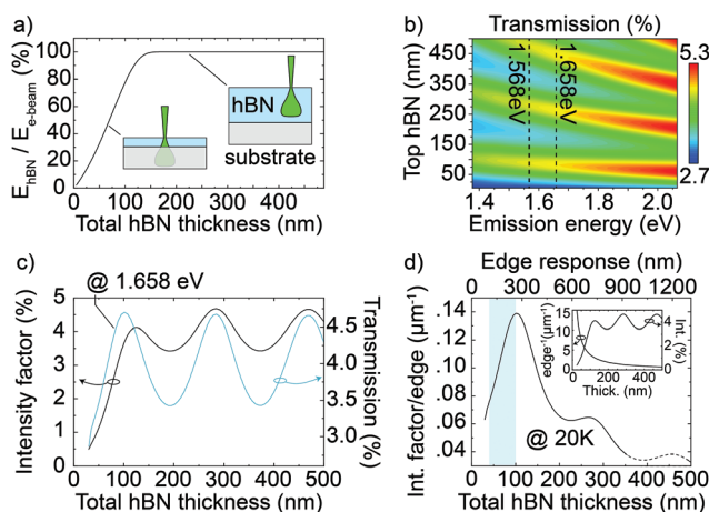
Fig. 4 (a) Energy deposited in hBN by a 3 kV e-beam as a function of the hBN thickness (Monte Carlo simulations). 100% corresponds to the whole e-beam energy deposited in hBN. (b) Three-dimensional Lumerical simulation of light transmission through top hBN as a function of the top hBN thickness between 10 nm and 500 nm (bottom hBN fixed at 20 nm). (c) Right axis: Transmission at 1.658 eV from the simulation in (b) as a function of the total hBN thickness (top and bottom). Left axis: CL intensity as a function of total hBN thickness obtained combining the curve in (a) with the transmission at 1.658 eV. (d) Inset: CL intensity from (c) (right axis) and the inverse of the edge response (left axis). Main: CL intensity from (c) divided by the edge response (linear fit in Fig. 2d) as a function of the total hBN thickness (bottom axis) and edge response (top axis). The blue shading indicates the range of optimization for brightness and resolution.
