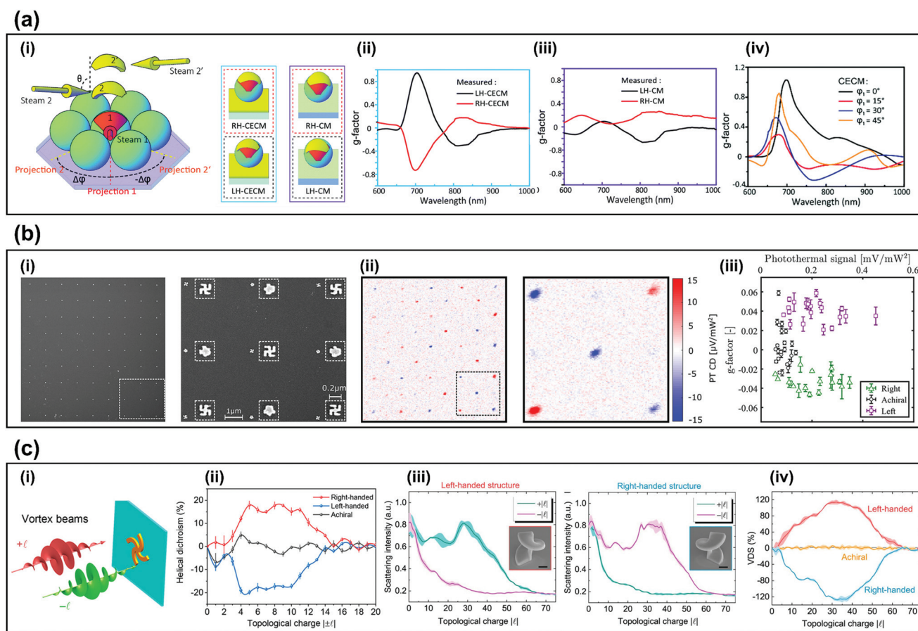
Fig. 3 Methods for sensitive chiral sensing. (a) CECM chiral signal. 20 (i) Schematic diagram of two-step ADMD on a self-assembled microsphere monolayer and schematic of RH-CECMs, RH-CMs, LH-CECMs, LH-CMs. (ii) Measured g factor of LH-CECM and RH-CECM that was fabricated to achieve \theta = 75^\circ , \Delta\phi = \pm 45^\circ . (iii) Measured g factor of LH-CM and RH-CM that was fabricated to achieve \theta = 75^\circ , \Delta\phi = \pm 45^\circ . (iv) Simulated g -factor of LH-CECMs that was fabricated to achieve \phi = 0^\circ (black), 15^\circ (red), 30^\circ (blue), and 45^\circ (magenta). (b) Chiral photothermal imaging. 18 (i) (left) SEM image of a 9 \times 9 gammadion array and (right) SEM image of the area surrounded by dashed square in (i). (ii) Photothermal dichroism image of (i) and (right) detailed photothermal dichroism image of the dashed part of (ii). (iii) g factor vs photothermal signal of 81 nanostructures that has three different handedness. (c) Measured and simulated HD of the nanostructures. 6,17 (i) Schematic of measuring HD illuminated by vortex beam. (ii) HD of the right and left achiral Archimedean spiral. (iii) Measured scattering spectra of left and right-handed helix structure illuminated by focused optical vortices. (iv) HD of the left, right and achiral nanostructure. (c) Reproduction with permission from Ref. 20. (c-iii, and iv) Reproduction with permission from Ref. 17. (c-i, and ii) Reproduction with permission from Ref. 6. (c-iii, and iv) Reproduction with permission from Ref. 17.
