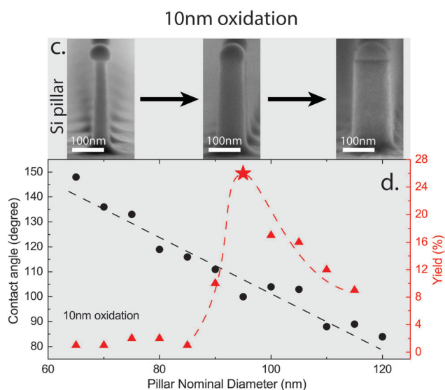
Fig. 2 Aspects and statistics of NW growths done on EBL-patterned SiO 2 /Si pillars. (a) SEM image (20° tilt) showing vertical GaAs NWs grown on SiO 2 /Si (111) pillars. (b) Vertical yield as a function of pillar nominal diameter. (c) SEM images showing Ga droplets on top of SiO 2 /Si pillars of different nominal diameters. (d) Contact angle and yield as a function of pillar nominal diameter for pillars as shown in c. The optimum contact angle is identified as the one showing the best vertical yield.
