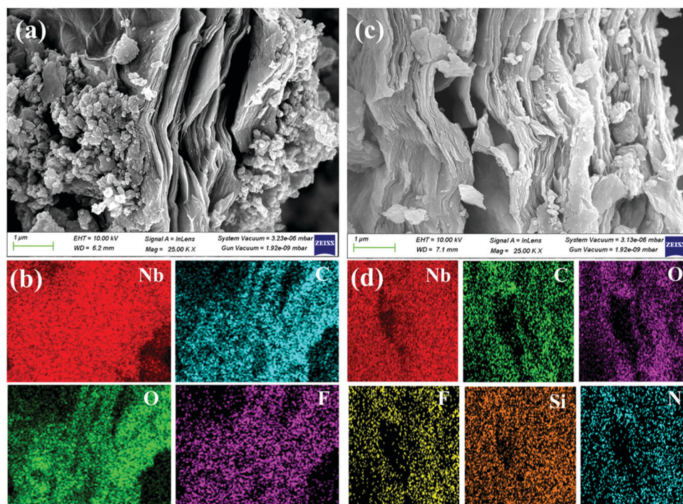
Fig. 4 FESEM and the corresponding elemental mapping of pristine \text{Nb}_2\text{CT}_x MXene (a and b) and \text{Nb}_2\text{CT}_x\text{-0.2 APTES} MXene (c and d).
