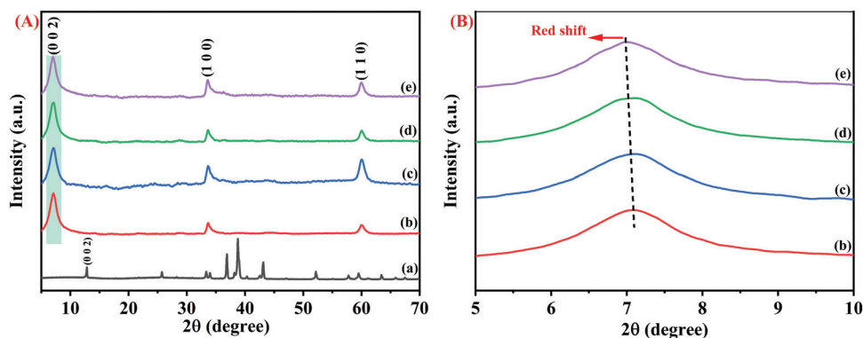
Fig. 3 (A) Full and (B) enlarged XRD of the \text{Nb}_2\text{AlC} MAX Phase (a), \text{Nb}_2\text{CT}_x MXene (b), \text{Nb}_2\text{CT}_x\text{-0.1 APTES} (c), \text{Nb}_2\text{CT}_x\text{-0.2 APTES} (d), \text{Nb}_2\text{CT}_x\text{-0.3 APTES} (e).
