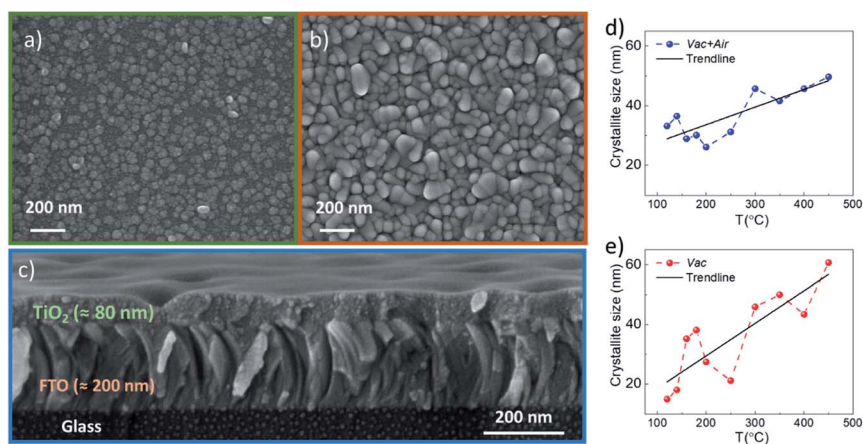
Fig. 2 (a and b) Top view SEM images of USP-deposited \text{TiO}_2 after a 160 ^\circ\text{C} vacuum annealing step (Vac) and after 160 ^\circ\text{C} vacuum and subsequently 450 ^\circ\text{C} air annealing steps (Vac+Air), respectively. (c) Cross-sectional view of the \text{TiO}_2 layer after 160 ^\circ\text{C} vacuum and subsequently 450 ^\circ\text{C} air annealing steps (Vac+Air). (d and e) Evolution of the crystallite size of vacuum and subsequently air annealed (labeled as Vac+Air) and vacuum annealed only (labeled as Vac) \text{TiO}_2 films.
