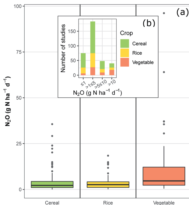
Fig. 2 (a) Boxplot of daily background nitrous oxide emissions (BNE) ( \text{g N}_2\text{O-N ha}^{-1} \text{ d}^{-1} ) from different crop categories (cereals, rice and vegetables) and (b) histogram of distribution of the daily BNE at these crop categories.
