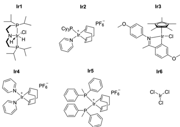
Fig. 155 Survey of Ir-based organometallics subject to pyrolysis with activated carbon. Ir1, Ir2, Ir3, Ir4, Ir5, and Ir6 correspond to the following organometallics, respectively: chlorodihydrido[bis(2-diisopropylphosphino)ethylamine]iridium(III), (1,5-cyclooctadiene)(pyridine)(tricyclohexylphosphine)iridium(I) hexafluorophosphate, chloro(5-methoxy-2-[(1-(4-methoxyphenyl)imino-N-methyl)phenyl-C](1,2,3,4,5-pentamethylcyclopentadienyl)iridium(III), bis(pyridine)(1,5-cyclooctadiene)iridium(I) hexafluorophosphate, (1,5-cyclooctadiene)bis(methyldiphenylphosphine)iridium(I) hexafluorophosphate, and iridium chloride. Reproduced with permission from ref. 1860 Copyright Wiley 2020.
