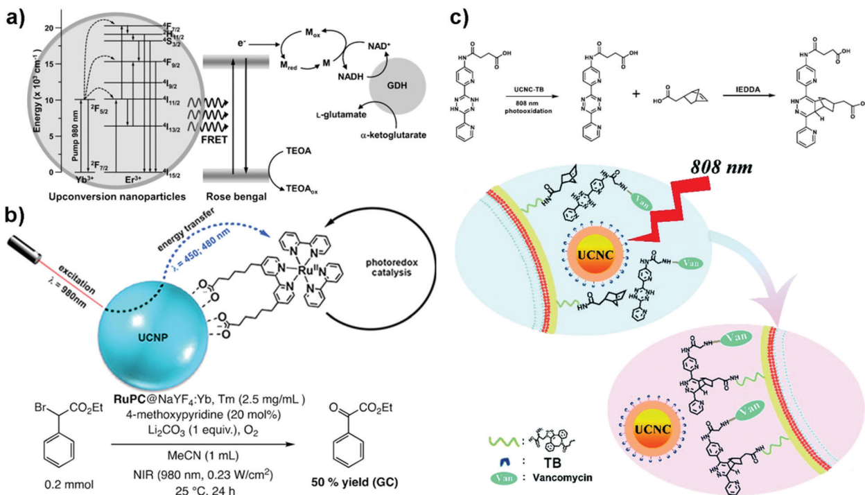
Fig. 3 (a) NIR-driven photoenzymatic catalysts combining NaYF 4 :Yb 3+ ,Er 3+ , Rose Bengal (RB), a rhodium(III)-based mediator (M), nicotinamide adenine dinucleotide (NAD + ) and L-glutamate dehydrogenase (GDH). 15 Reprinted with permission from ref. 15. Copyright 2014, Wiley-VCH. (b) NIR-driven photocatalyst combining NaYF 4 :Yb 3+ , Tm 3+ and a heteroleptic derivative of [Ru(bpy) 3 ] 2+ . 16 Reprinted with permission from ref. 16. Copyright 2018, Wiley-VCH. (c) NIR-driven photocatalyst combining NaYF 4 :Nd 3+ ,Yb 3+ ,Er 3+ @NaYF 4 :Nd 3+ and Toluidine Blue O (TB). 17 Reprinted with permission from ref. 17. Copyright 2021, Royal Society of Chemistry.
