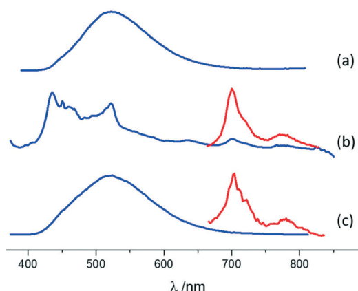
Fig. 6 Normalized luminescence spectra in the solid state of (a) pure MA, (b) MA \cdot I2F4 , and (c) (MA)_4 \cdot I2F4 (arbitrary units on the y-axis). \lambda_{exc} = 380\ nm . The phosphorescence spectra in the 650–850 nm region, isolated with a gated detection, are magnified in the inset for MA \cdot I2F4 and (MA)_4 \cdot I2F4 . In both co-crystals the phosphorescence emission is clearly evidenced compared to the parent PAH 9-methylanthracene, where no phosphorescence was detected at all. Moreover, for MA \cdot I2F4 the spectrum is not dominated by excimer emission.
