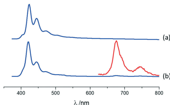
Fig. 5 Normalized luminescence spectra in the solid state for (a) pure A and (b) A \cdot (I2F4)_2 (arbitrary units on the y-axis). \lambda_{exc} = 380\ nm . The phosphorescence spectrum in the 650–800 nm region, isolated with a gated detection, is magnified in the inset for A \cdot (I2F4)_2 . The phosphorescence emission is clearly evident in A \cdot (I2F4)_2 compared to solid anthracene, where no phosphorescence was detected.
