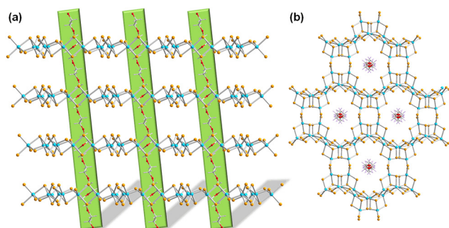
Fig. 6 The infinite PEG polymer strands running through the hexagonal nanochannels of 2D- [\text{Sn}_3\text{Se}_6(\text{Se}_2)]^{2-} layers, viewed along different crystallographic direction in (a and b). Hydrogen atoms and counterions are omitted for clarity. Color code: Sn-turquoise, Se-orange, C-grey, O-red.
