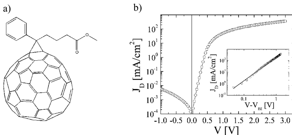
Fig. 8 (a) Chemical structure of [84]PCBM. (b) Dark current density–voltage characteristics ( J_D ) of an ITO/PEDOT:PSS/[84]PCBM:MDMO-PPV(4 : 1 w/w)/LiF/Al diode with a thickness of 129 nm at a temperature T = 295 K. The inset shows the \log(J_D) – \log(V) characteristic corrected for the built-in voltage ( V_{bi} = 0.31 V), together with the calculated SCLC (solid line) (replotted with permission from ref. 32. Copyright 2006 American Chemical Society).
