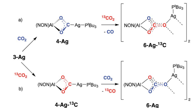
Fig. 9 ^{13}\text{CO}_2 'crossover' labelling experiments (and their associated spectra) carried out with 4-Ag and 4-Ag- ^{13}\text{C} : (a) addition of ^{13}\text{CO}_2 to 4-Ag to yield 6-Ag- ^{13}\text{C} and \text{CO} ; (b) addition of unlabelled \text{CO}_2 to 4-Ag- ^{13}\text{C} to yield 6-Ag and ^{13}\text{CO} .
