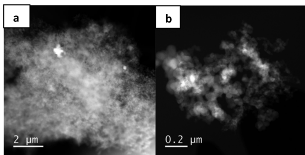
Fig. 2 Selected HAADF-STEM images of fresh Cu-phen/C-800. The fresh catalyst contains a few very large Cu containing particles (a), while in most parts of the material no Cu particles are visible at all (b).
