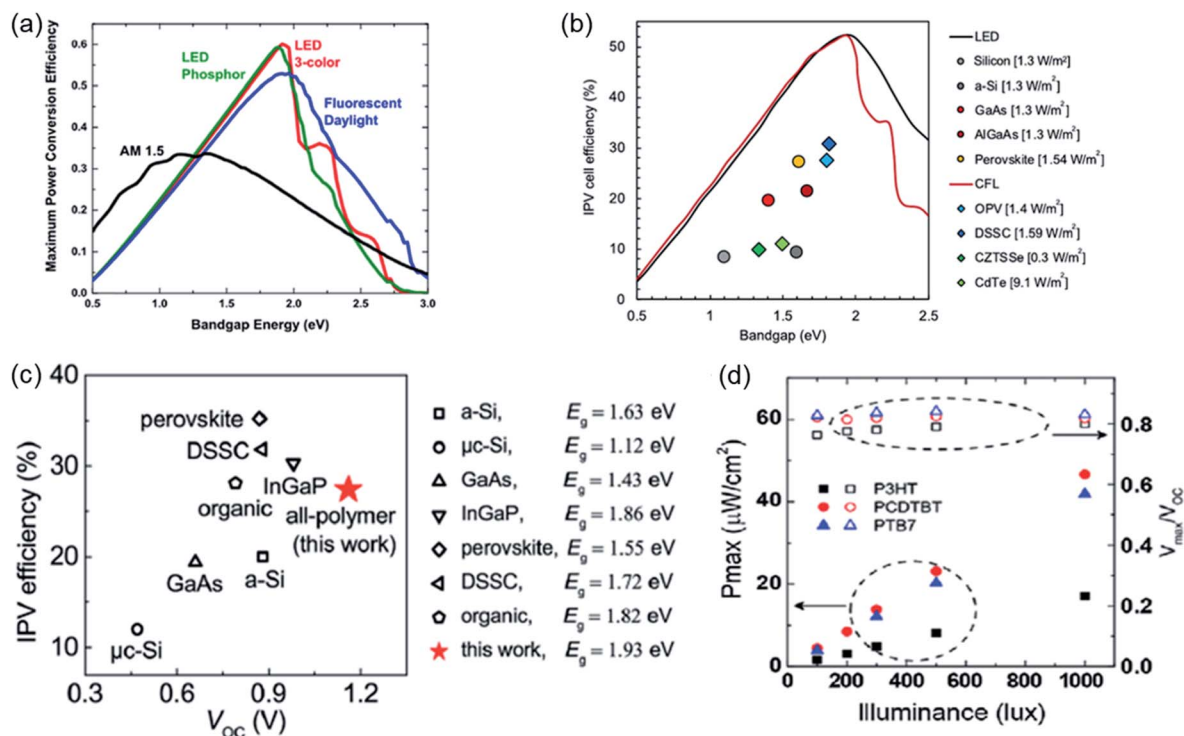
Fig. 2 (a) The bandgap of the light-absorbing layer material under different light sources and the maximum photoelectric conversion efficiency of the corresponding IPV. Reproduced from ref. 24 with permission from the [Institute of Electrical and Electronics Engineers Inc], copyright [2015]. (b) The statistics of maximum efficiency (under CFL and LED illumination) and bandgap for IPVs, so far. Reproduced from ref. 45 with permission from the [Elsevier], copyright [2018]. (c) The PCE and V_{OC} distribution of various types IPVs under the indoor light source. Reproduced from ref. 96 with permission from the [Royal Society of Chemistry], copyright [2019]. (d) OPVs maximum power output density and V_{max}/V_{OC} ratio under indoor light source. Reproduced from ref. 77 with permission from the [American Institute of Physics], copyright [2016].
