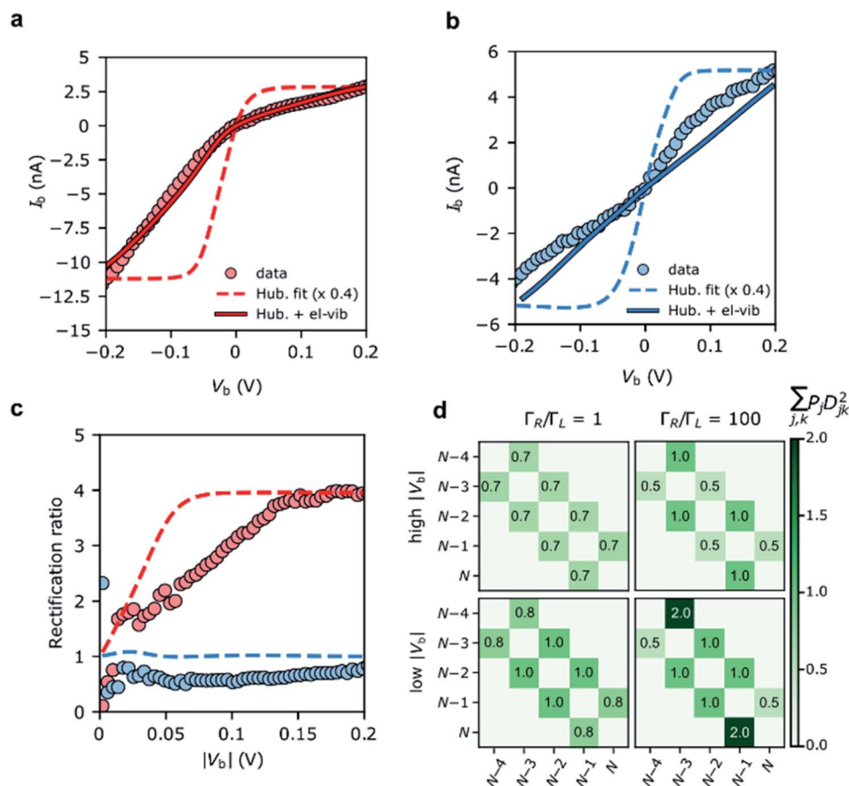
Fig. 4 Device I/V traces on (a) the N - 4/N - 3 resonance ( V_g = -66 V), and (b) the N - 3/N - 2 resonance ( V_g = -34 V). The experimental data are plotted alongside I/V traces taken from the Hubbard stability diagrams in Fig. 3, and the Hubbard model plus electron–vibration coupling included in the electron-transfer rates. Electron–vibration fitting parameters for N - 4/N - 3 : \Gamma_L = 41 \mu eV, \Gamma_R = 14 meV, \lambda_0 = 70 meV; for N - 3/N - 2 , \lambda_0 = 120 meV. (c) The rectification behaviour, I_b(-V_b)/I_b(+V_b) , of the N - 4/N - 3 (red) and N - 3/N - 2 (blue) transitions are given for the experimental values (circles) and the Hubbard model (dashed lines). The measurements were taken at a device temperature of 77 K. (d) The emergence of the rectification behaviour of the Hubbard model under asymmetric molecule–electrode coupling. Each element ( j, k ) represents the sum of the electron transfer rates from charge state j to k . ‘High’ |V_b| means above 2|t|/\alpha_S , when both N - 3 doublets are within the bias window. An improved fit to N - 3/N - 2 (maintaining the rectification ratio) can be achieved by going beyond the wide-band gap approximation, see ESI.†
