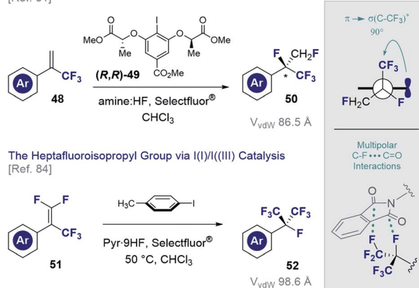
Fig. 12 Generating fluorinated surrogates of the isopropyl group via l )/ l catalysis.
