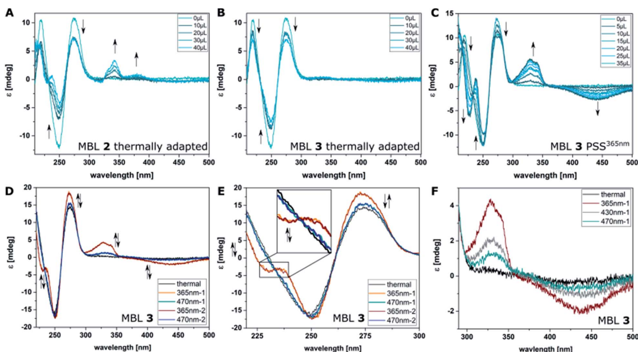
Fig. 7 Binding studies using CD spectroscopy by titrating increasing amounts of MBLs 2 (A), and 3 (B) to dsDNA (5′-d(CTAACGGAATG)-3′/3′-d(GATTGGCTTAC)-5′, 5 \mu M) in phosphate buffer at their thermal equilibrium and of 3 at the PSS 365nm (C). (D) CD spectra of compound 3 (10 \mu M) in the presence of dsDNA (5 \mu M) in phosphate buffer. Altering irradiation with 365 nm and 470 nm light and reversible structural change in DNA and of the ICD of 3 . (E) Excerpt showing the reversible structural change in the DNA-region of the CD spectra. (F) Irradiation of MBL 3 with different colors of light: CD spectrum at the thermal equilibrium (black), the PSS 365nm (red), the PSS 430nm (grey), and the PSS 470nm (cyan) containing varying amounts of Z isomer (a wider spectral range can be found in Fig. S30†).
