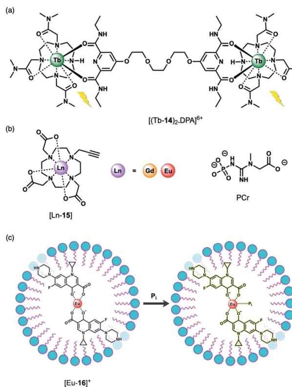
Fig. 7 (a) Tb(III)-Based displacement assay for \text{HPO}_4^{2-} and \text{NO}_3^- ; (b) alkyne-functionalised DO3A complex for assessing bulk phosphate species (PCr, \text{HPO}_4^{2-} ); (c) schematic depiction of the detection of \text{HPO}_4^{2-} ( \text{Pi} ) in water samples, using a Eu(III)-CIP mixture in the presence of the surfactant SDBS.
