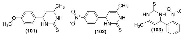
Fig. 28 Chemical structures of 4-phenylpyrimidine-2(1H)-thiones ( 101–103 ).
