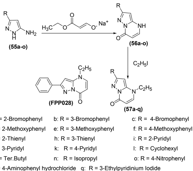
Scheme 24 Synthesis of pyrazolo[l,5-a]pyrimidin-7-ones (57a–q).
